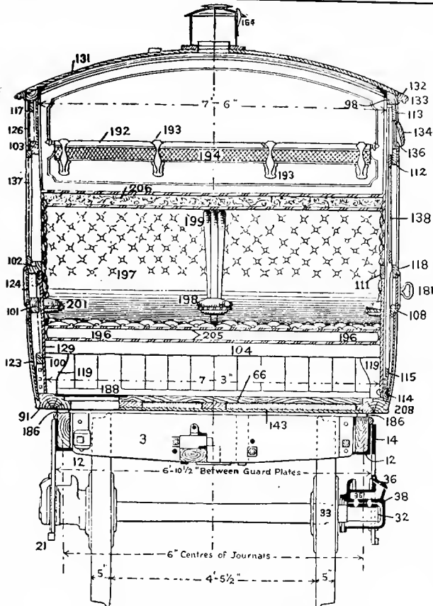
Fig. 503. Transverse Section.
